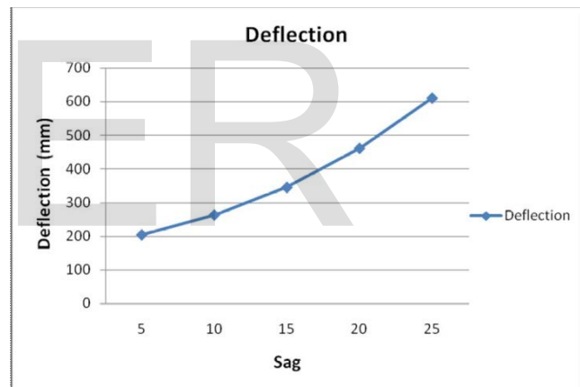
Fig 21: variation of girder deflection with sag of main cable
